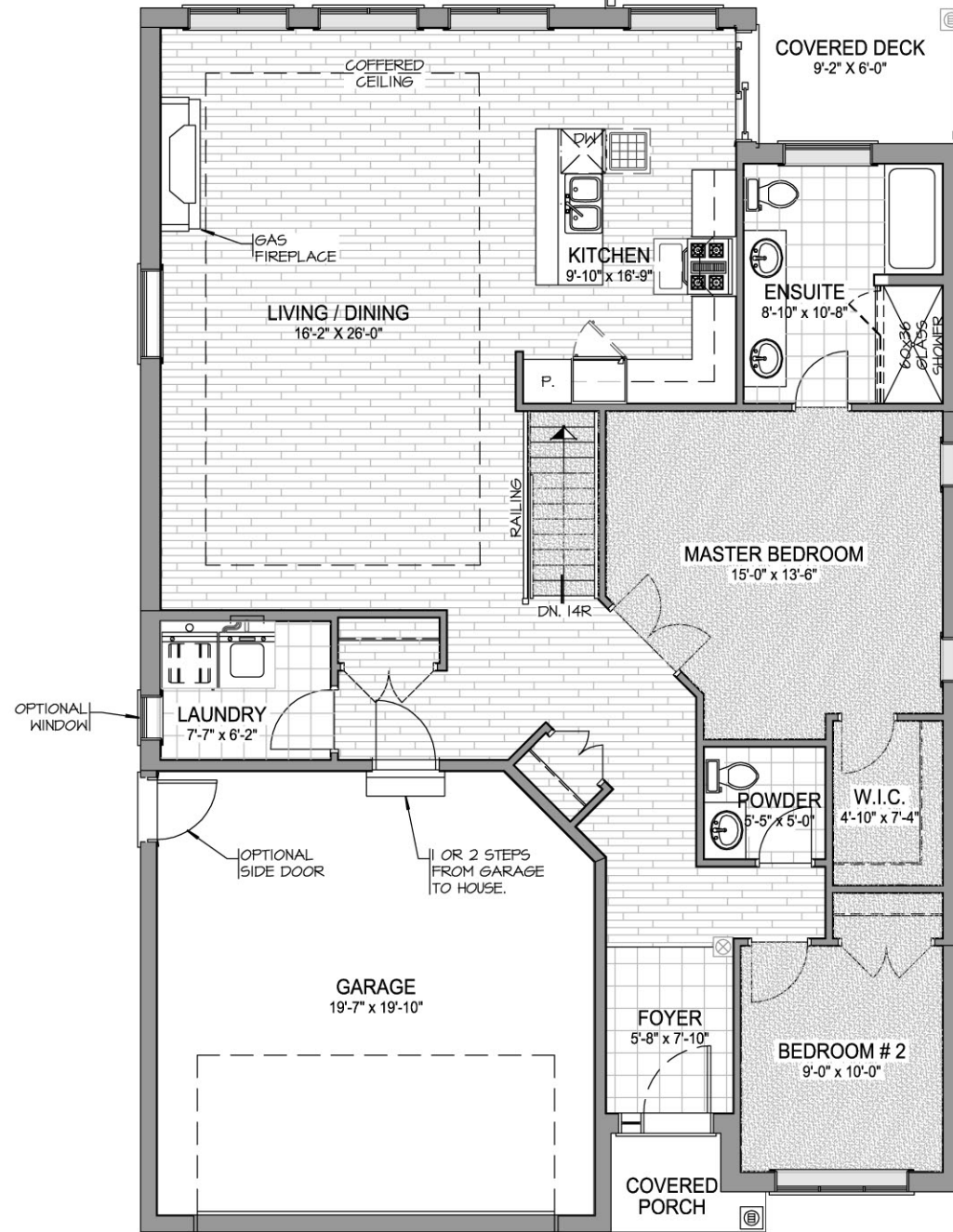
Main Floor Plan (1507 sq.ft.)
