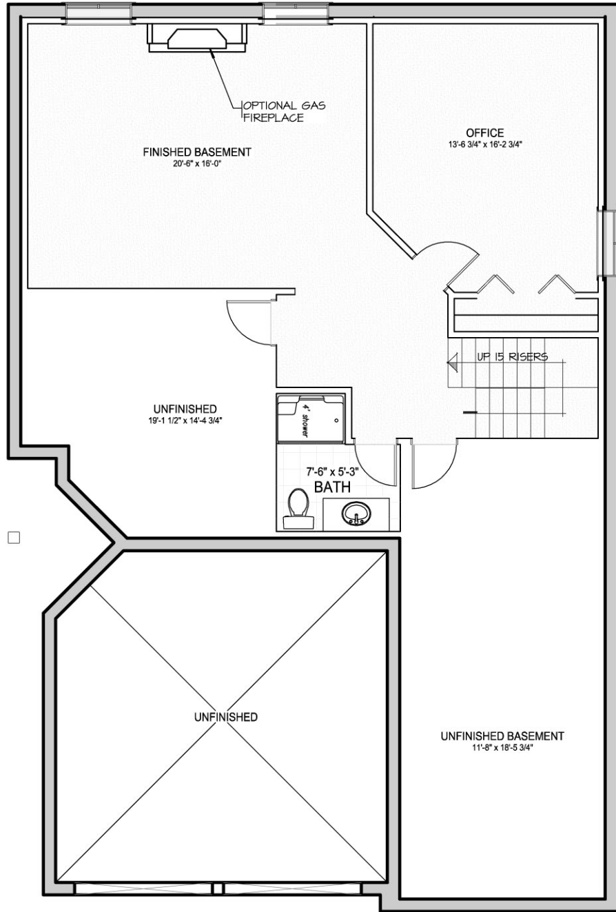
Basement Floor Plan (775 sq.ft.)
