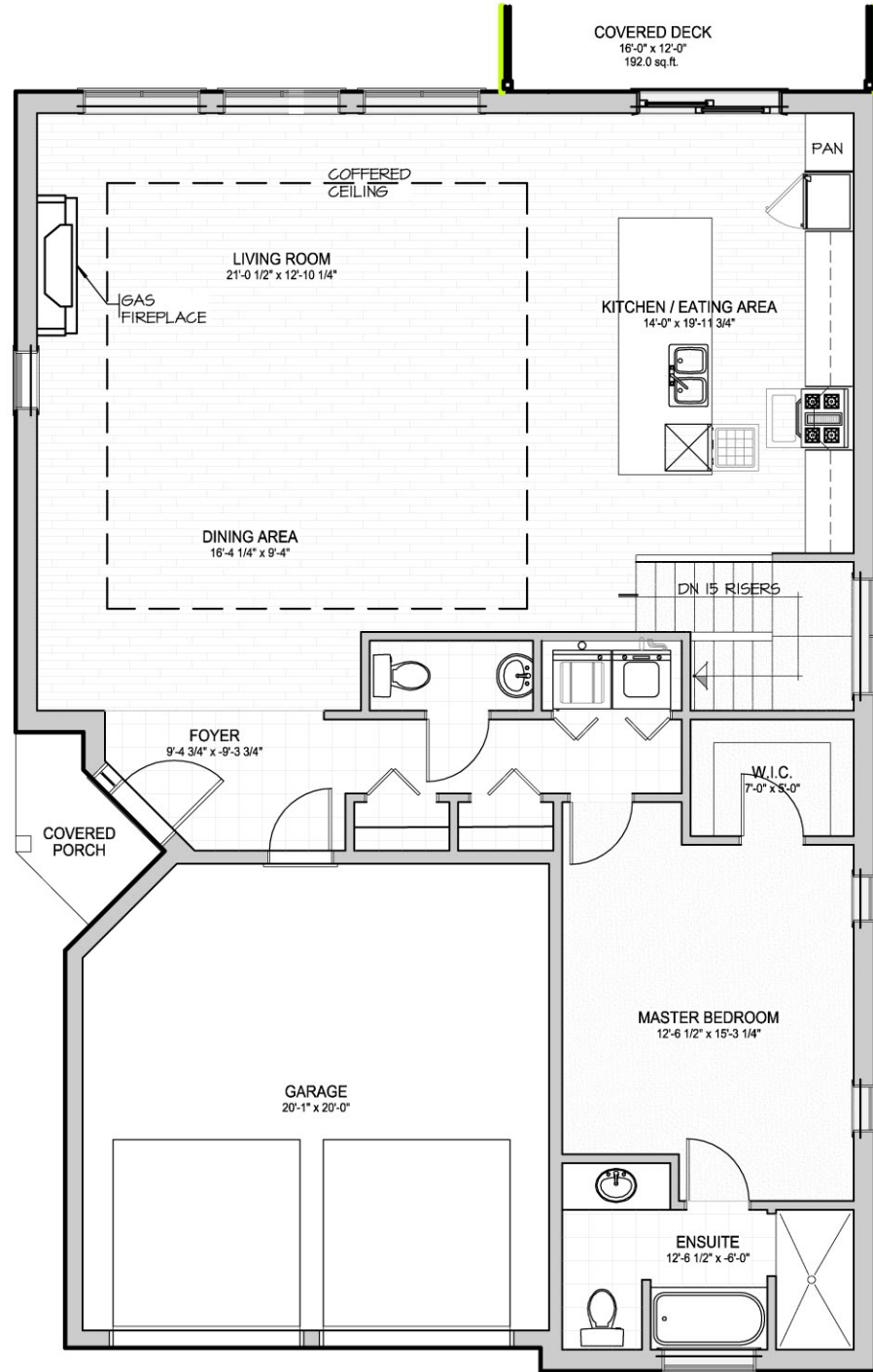
Main Floor Plan (1499 sq.ft.)
